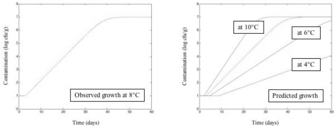
Figure 4. An example of a predictive microbiology.
